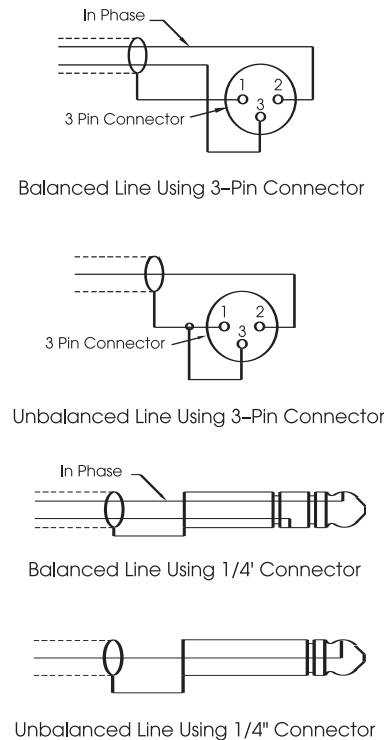
Figure 5: Audio Connection
